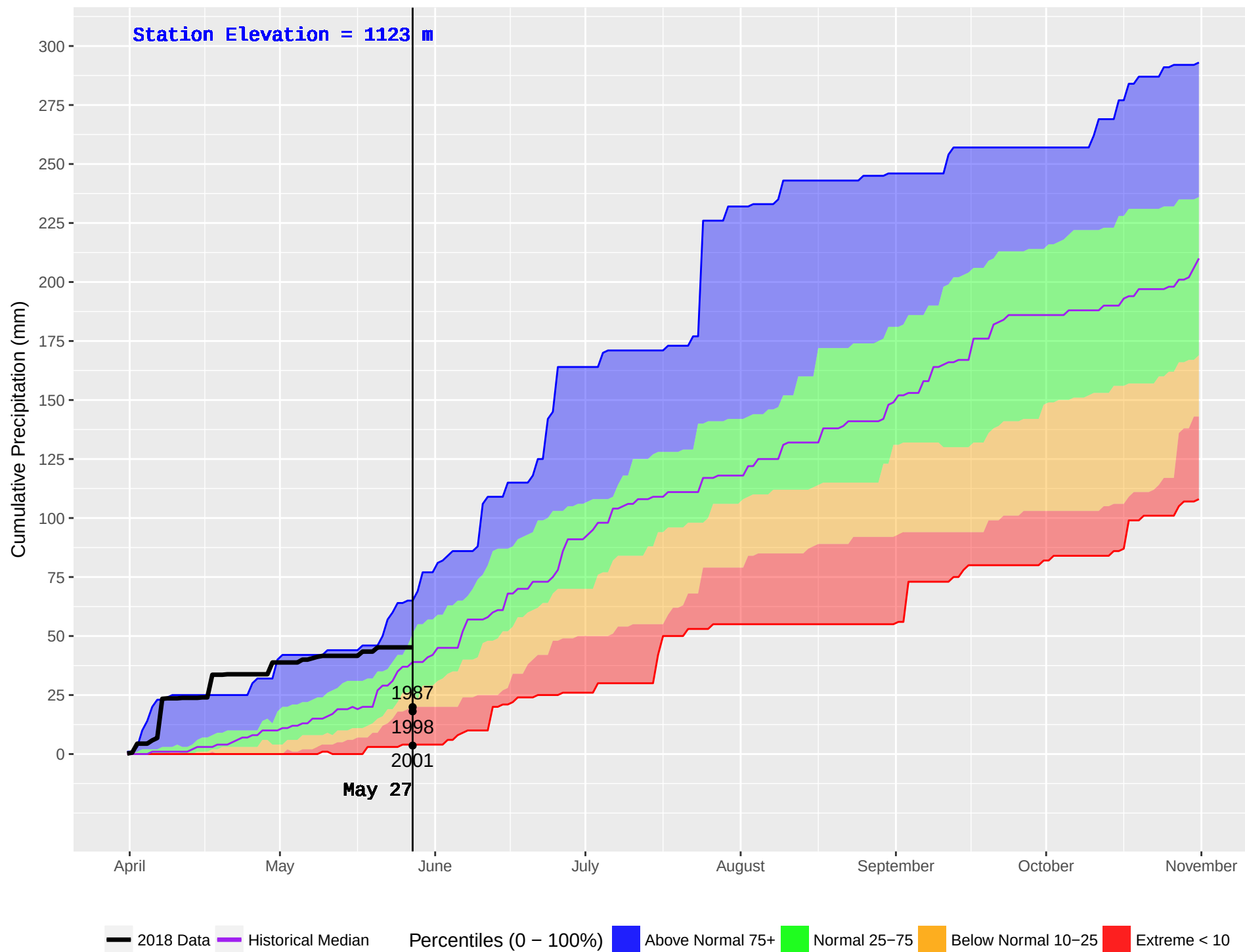
MCLEAN LAKE (311) : Historical (1987–2016) and Current (2018) Noon Cumulative Precipitation
