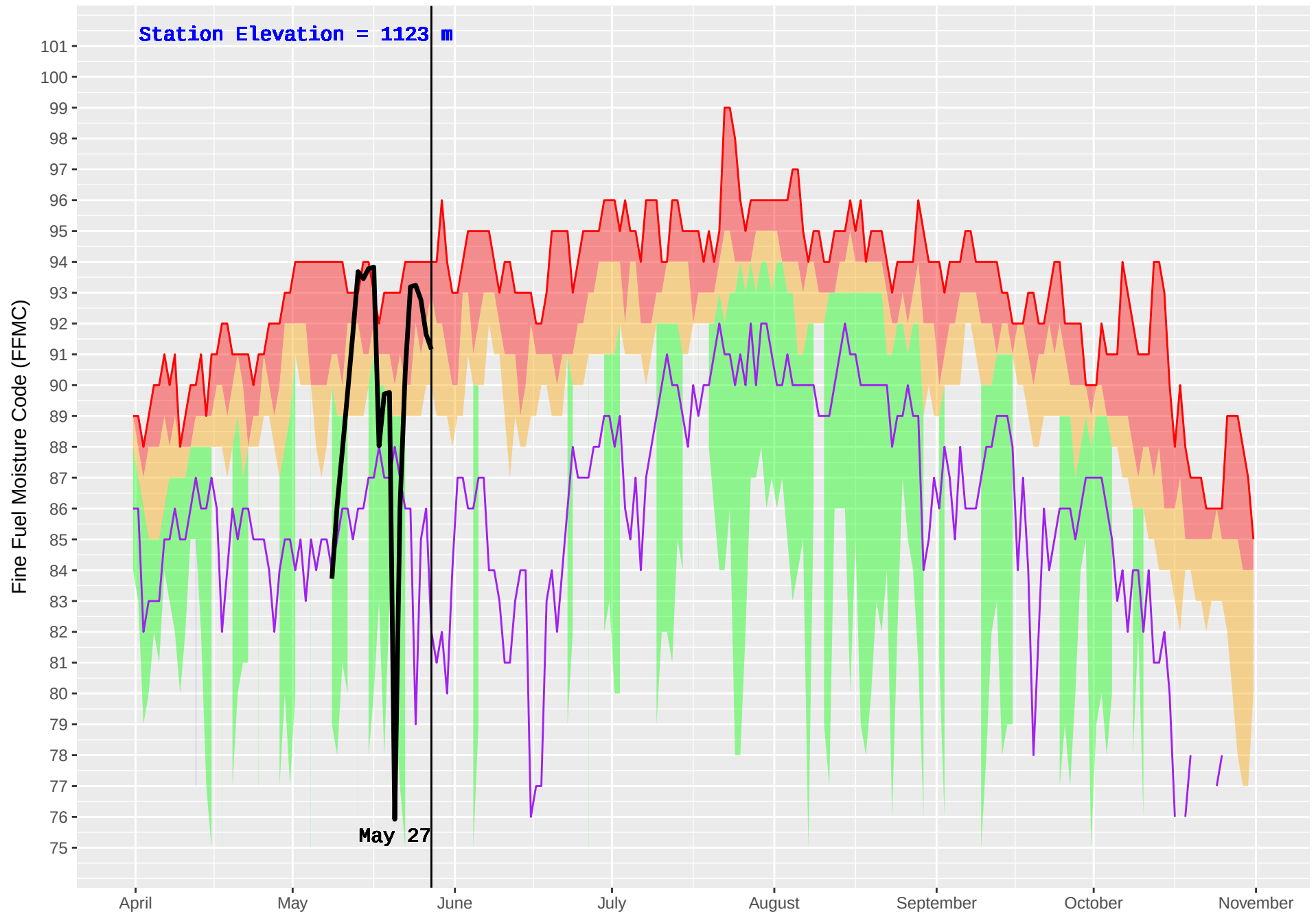
MCLEAN LAKE (311) : Historical (1987–2016) and Current (2018) Noon Fine Fuel Moisture Code (FFMC)
